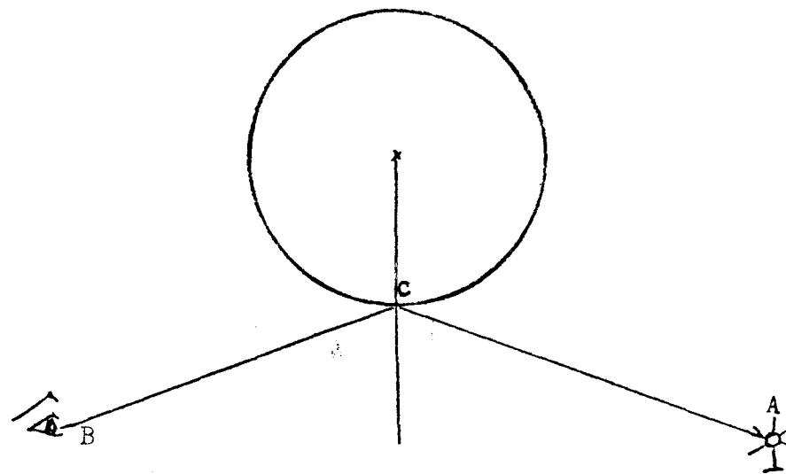
Fig. 5. The famous problem of Alhazen (Ibn al-Haytham). Given a light source at A and observer at B, find point C on a cylindrical mirror such that the light ray will be reflected to the observer at B.
