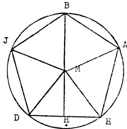
Fig. 4. Reproduced from Abu Kamil's "The Pentagon and the Decagon". Given the side of a regular pentagon, find the diameter.
